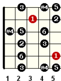
D Gypsy Minor Scale
