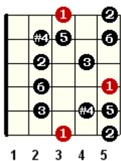
G Gypsy Minor Scale
