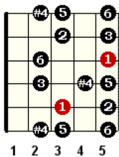
C Gypsy Minor Scale
