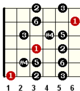
F Gypsy Minor Scale
