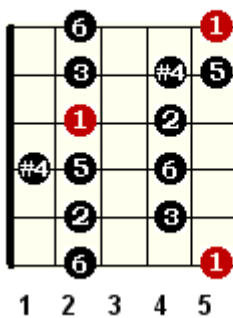
A Gypsy Minor Scale
